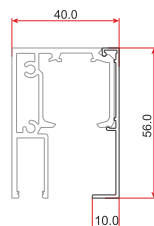
TOP TRACK COVER
