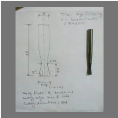
Carbide Dovetail Cutter
