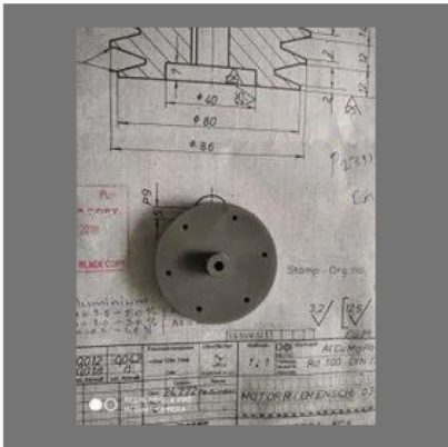
Carbide Punch & Stopper
