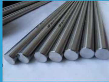
Titanium Ti-6Al-4V ELI (Grade 23) Bars
