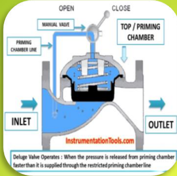
AUTO DELUGE VALVE
